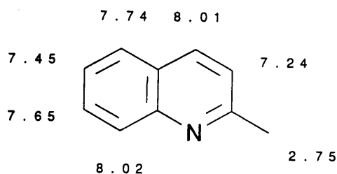
Figure 5 NMR Spectrum of Quinaldine prepared from D-5 Aniline by Döbner-Miller synthesis using deuterium chloride
